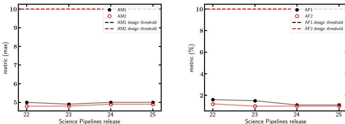
FIGURE 2: Astrometry metrics measured on r -band images compared over the past few major pipelines releases. Left: Median astrometric measurement error on 5-arcminute scales (AM1) and 20-arcminute scales (AM2), compared against the SRD requirements (for the “design” thresholds; note that the thresholds for AM1 and AM2 are the same, and thus indistinguishable on the figure). Right: Fraction of astrometric measurements exceeding the outlier threshold on 5-arcminute (AF1) and 20-arcminute (AF2) scales, compared against the SRD requirements (for the “design” thresholds; note that the thresholds for AF1 and AF2 are the same, and thus indistinguishable on the figure). The measured values of these metrics were virtually unchanged between pipelines version 24 and v25, as expected since no major changes have been made to astrometric measurement algorithms between v24 and v25.
